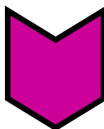
hexagon
