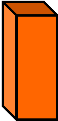
cuboid
