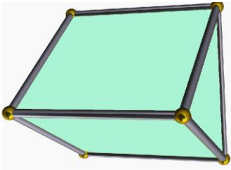
prism
