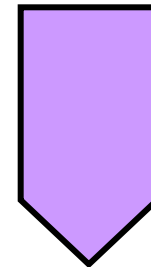
pentagon
