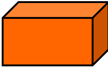
cuboid
