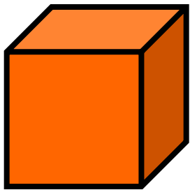
cube
