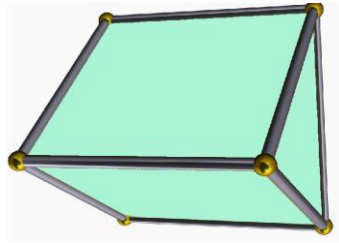
prism
