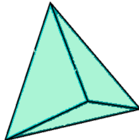
tetrahedron
