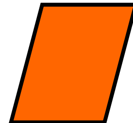
parallelogram
