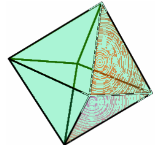
octahedron
