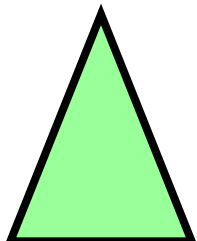
isosceles triangle
