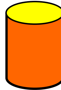
cylinder
