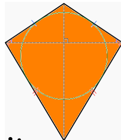
kite
