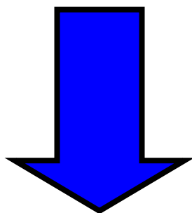
heptagon
