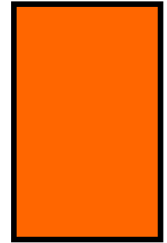
oblong/ rectangle
