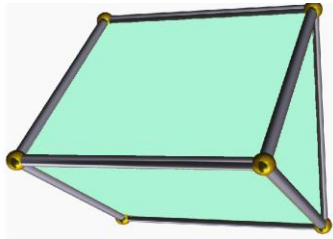
prism
