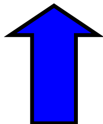
heptagon
