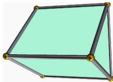
prism
