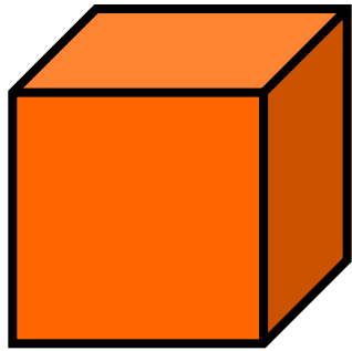
cube
