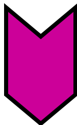
hexagon
