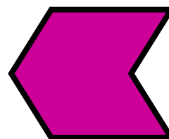
hexagon
